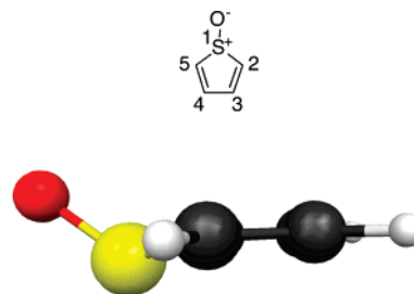
FIGURE 1. Out-of-plane sulfur geometry at MP2/6-31G(d,p).
